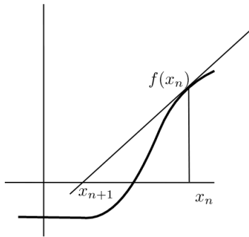
Figure 18.1: One step in the one-dimensional Newton method.
