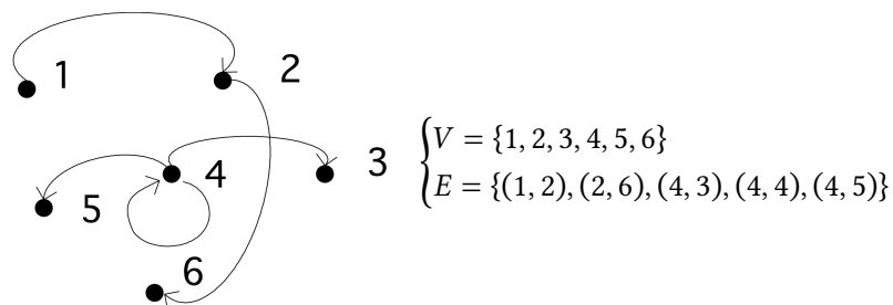
Figure 20.1: A simple graph.
