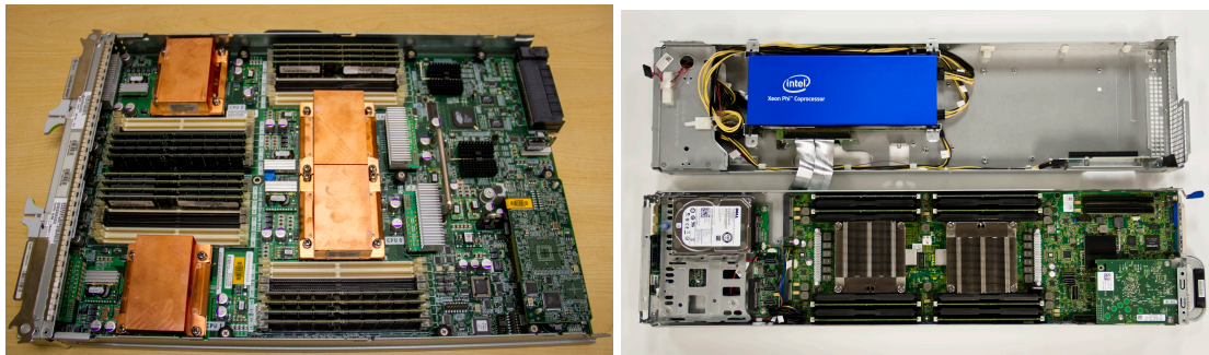
Figure 1.17: Left: a four-socket design. Right: a two-socket design with co-processor.
