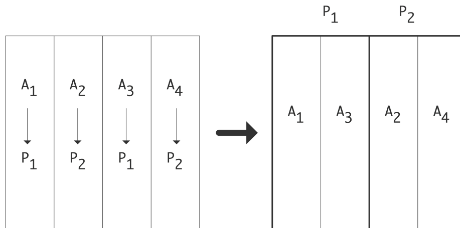
Figure 7.6: One-dimensional cyclic distribution: assignment of four matrix columns to two processors, and the resulting mapping of storage to matrix columns.
