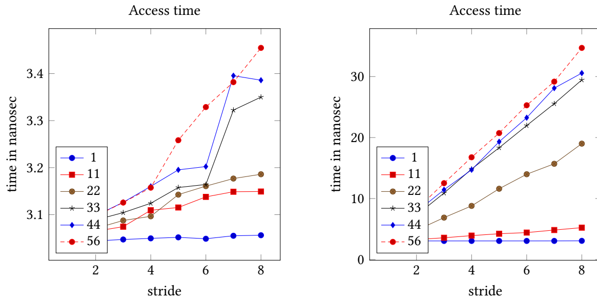
Figure 6.2: Access time per word for different strides and core counts, Frontera; dataset size left: 100k, right 1M; note different y scales!
