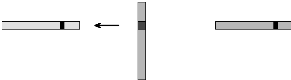
Figure 7.9: The block-panel multiplication in the matrix-matrix algorithm
