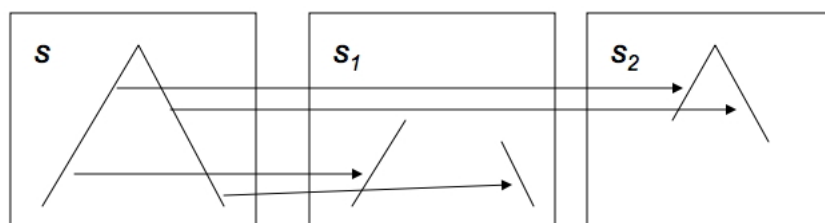
Figure 9.3: Illustration of a splitting a bitonic sequence.
