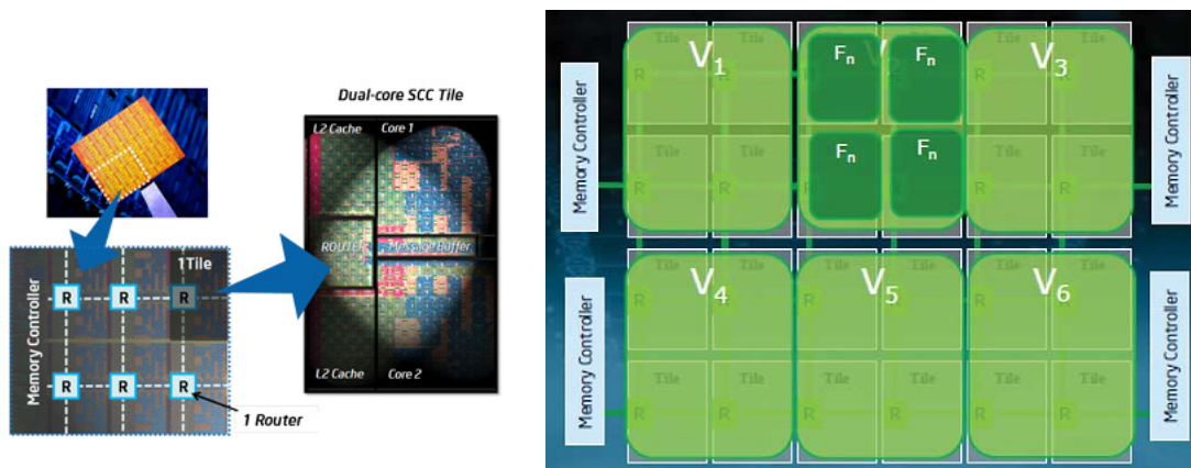
Figure 1.16: Structure of the Intel Single-chip Cloud Computer chip.
