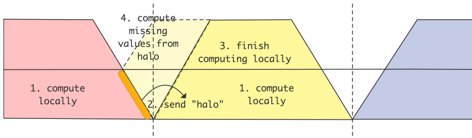
Figure 7.30: Computation of blocks of grid points over multiple iterations.
