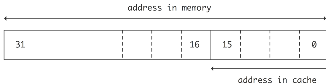
Figure 1.9: Direct mapping of 32-bit addresses into a 64K cache.
