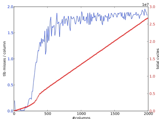
Figure 6.6: Number of TLB misses per column as function of the number of columns; columnwise traversal of the array.
