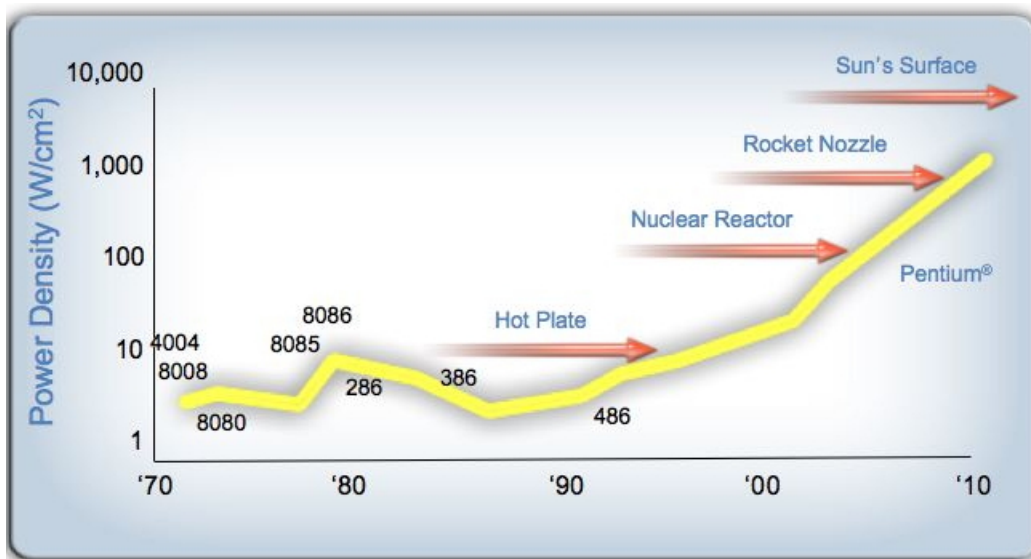
Figure 1.20: Projected heat dissipation of a CPU if trends had continued – this graph courtesy Pat Helsing.
