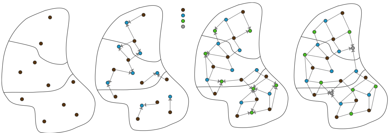
Figure 7.25: Solving a parallel multicolor ILU in four steps.
