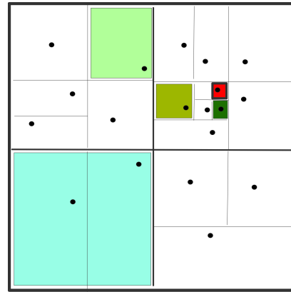
Figure 11.3: Boxes with constant distance/diameter ratio.
