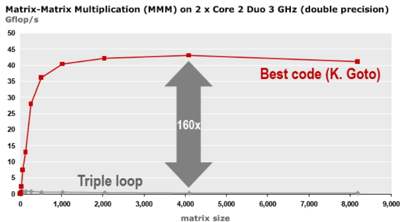
Figure 6.11: Performance of naive and optimized implementations of the matrix-matrix product.
