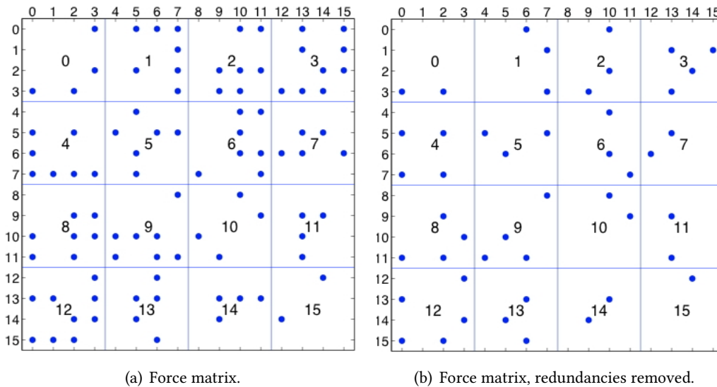
Figure 8.3: Force decomposition, showing a force matrix of 16 particles and forces partitioned among 16 processors.
