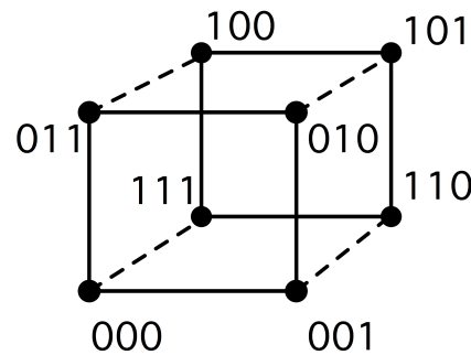
Figure 2.25: Gray code numbering of the nodes of a hypercube.
