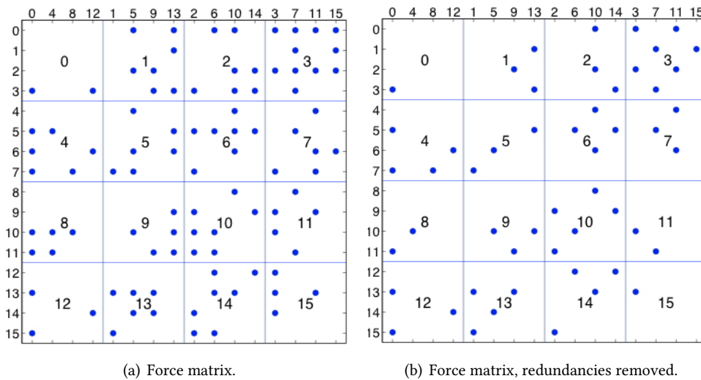
Figure 8.4: Force decomposition, with permuted columns in the force matrix. Note that columns 3, 7, 11, 15 are now in the block column corresponding to processors 3, 7, 11, 15 (the same indices), etc.
