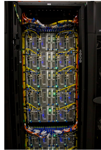
Figure 2.30: A fat tree with a three-level interconnect (left); the leaf switches in a cabinet of the Stampede cluster (right).
