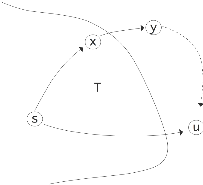
Figure 10.1: Illustration of the correctness of Dijkstra's algorithm.
