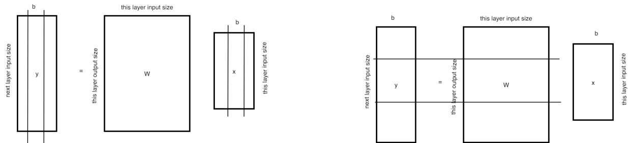
Figure 13.3: Partitioning strategies for parallel layer evaluation.
