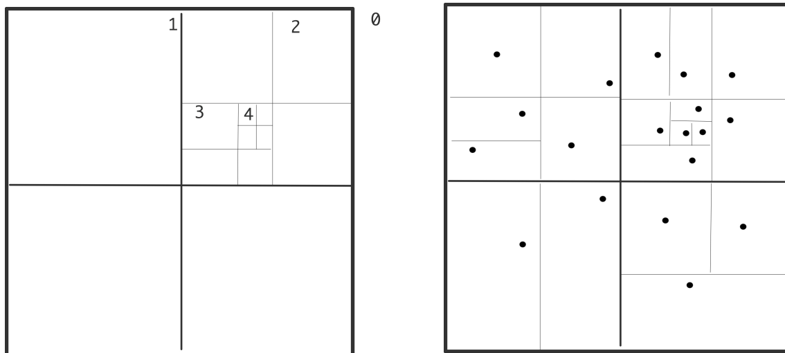
Figure 11.2: Recursive subdivision of a domain in quadrants with levels indicated (left); actual subdivision with one particle per box (right).
