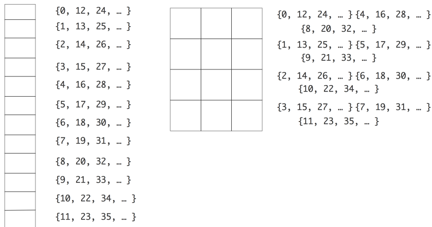
Figure 1.11: Two caches of 12 elements: direct mapped (left) and 3-way associative (right).
