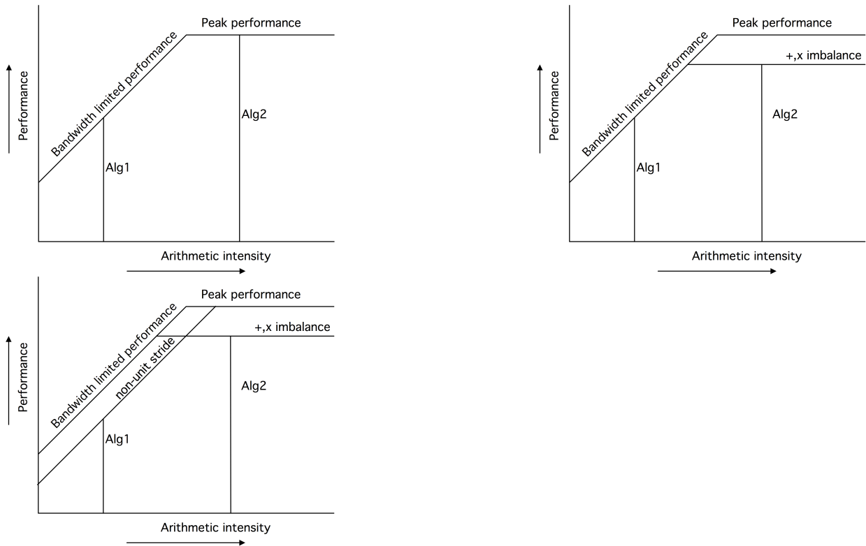
Figure 1.18: Illustration of factors determining performance in the roofline model.
