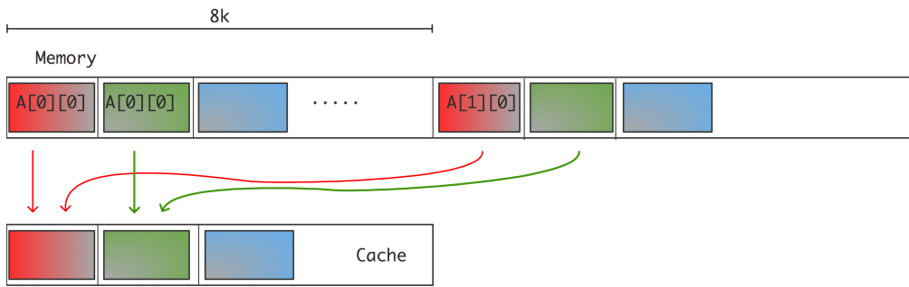
Figure 1.10: Mapping conflicts in direct mapped cache.
