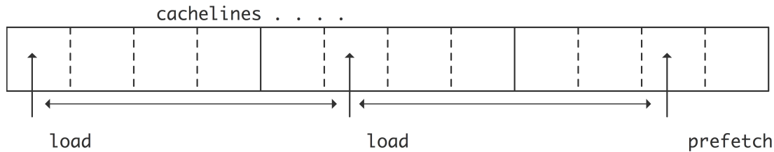
Figure 1.13: Prefetch stream generated by equally spaced requests.
