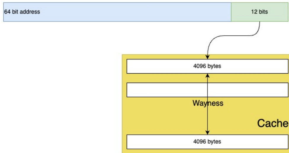
Figure 1.12: Associative cache structure
