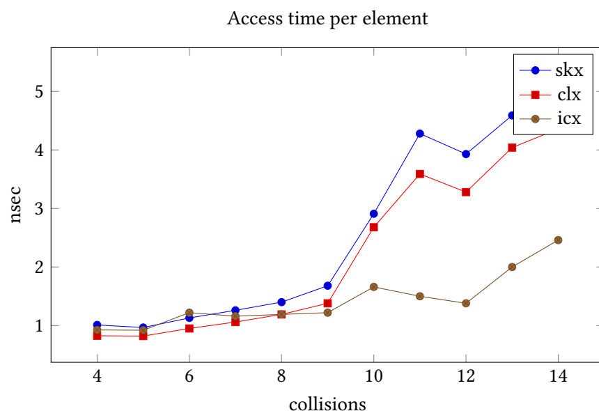
Figure 6.8: Effects of cache associativity
