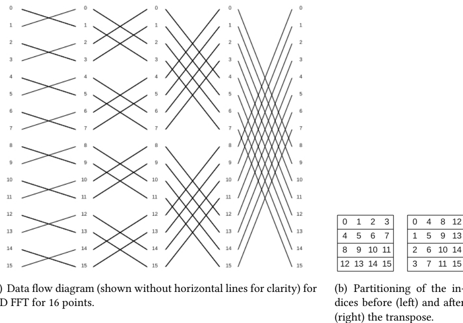
Figure 8.8: 1-D FFT with transpose. The first two stages do not involve communication. The data is then transposed among the processors. As a result, the second two stages also do not involve communication.
