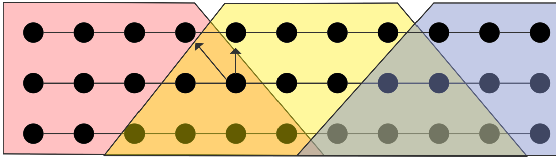
Figure 7.28: Computation of blocks of grid points over multiple iterations.
