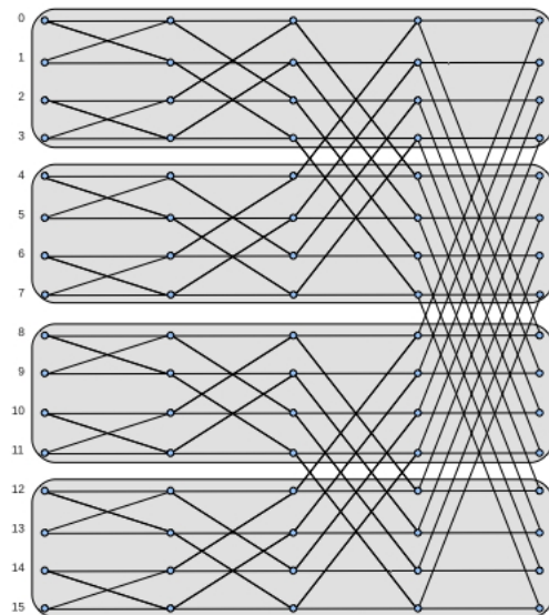
Figure 8.7: Data flow diagram for 1-D FFT for 16 points. The shaded regions show a decomposition for 4 processors (one processor per region). In this parallelization, the first two FFT stages have no communication; the last two FFT stages do have communication.
