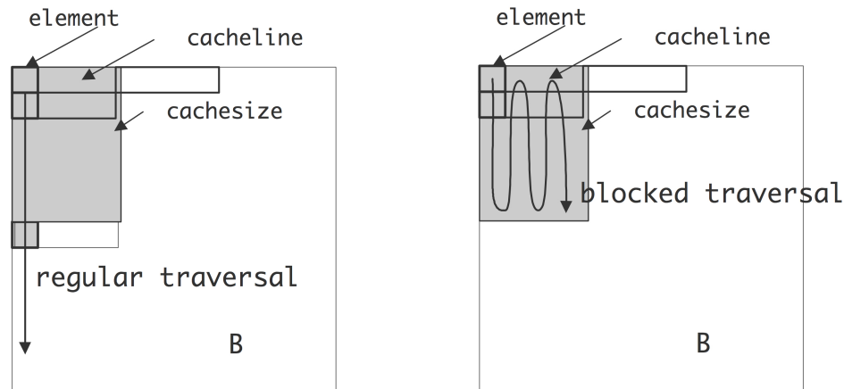
Figure 6.9: Regular and blocked traversal of a matrix.
