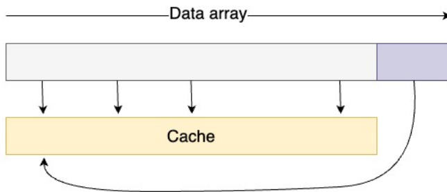
Figure 1.6: Illustration of a capacity miss
