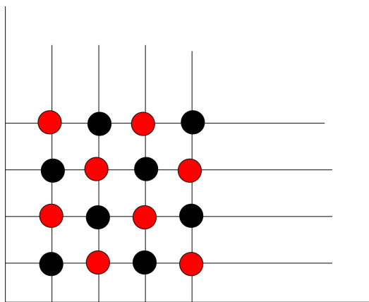
Figure 7.23: Red-black ordering of the variables of a two-dimensional domain.
