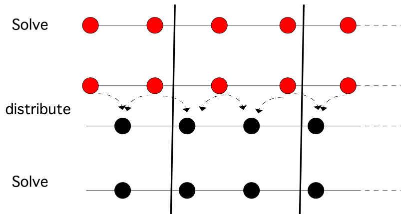
Figure 7.22: Parallel red-black solution on a 1d domain.
