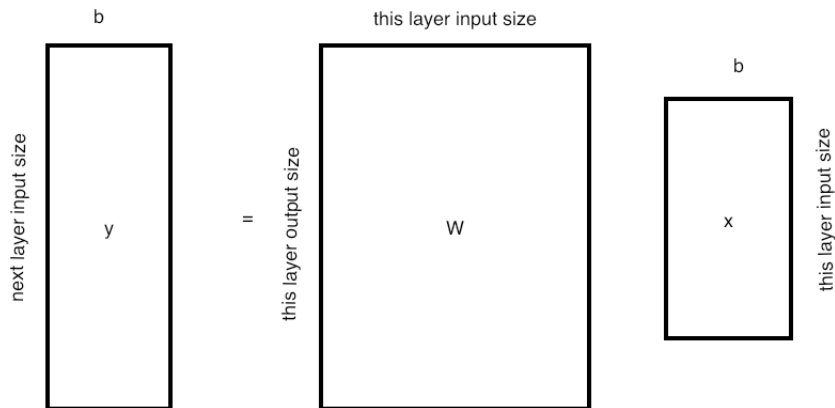
Figure 13.2: Shapes of arrays in a single layer.
