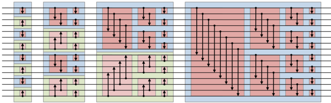
Figure 9.5: Full bitonic sort for 16 elements.
