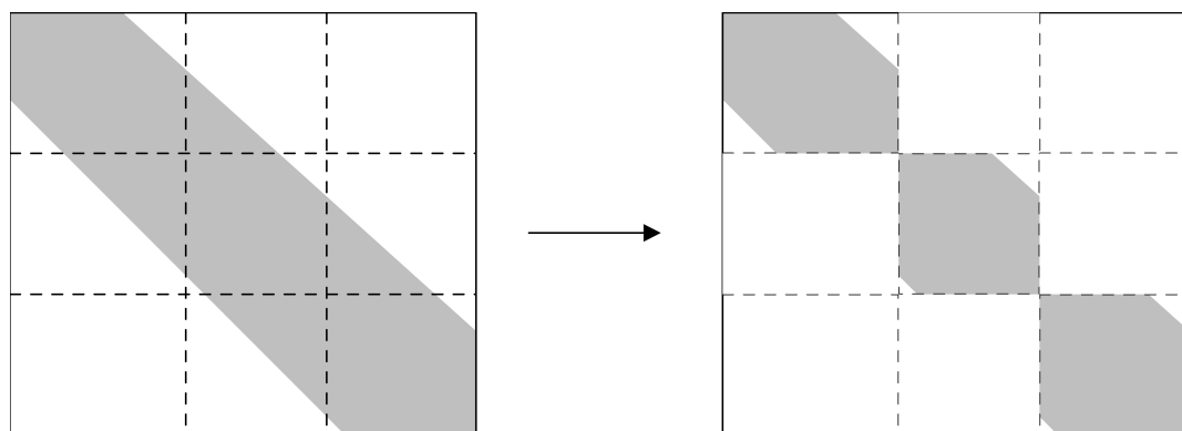
Figure 7.16: Sparsity pattern corresponding to a block Jacobi preconditioner.
