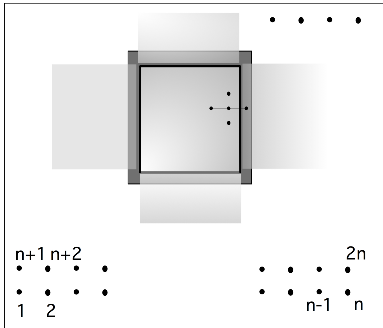
Figure 7.13: The ghost region of a processor, induced by a stencil.
