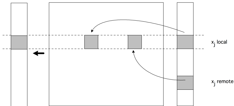
Figure 7.2: The parallel matrix-vector product with a blockrow distribution.
