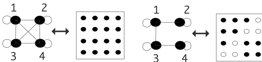
Figure 20.3: A dense and a sparse matrix, both with their adjacency graph.
