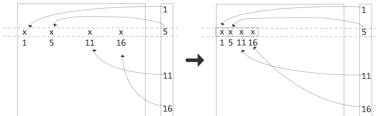
Figure 5.3: Compressing a row of a sparse matrix in the CRS format.
