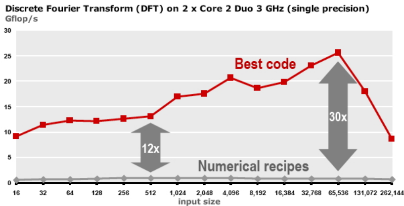
Figure 6.10: Performance of naive and optimized implementations of the Discrete Fourier Transform.
