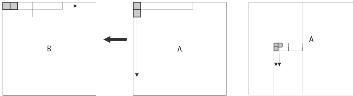
Figure 6.12: Matrix transpose operation, with simple and recursive traversal of the source matrix.
