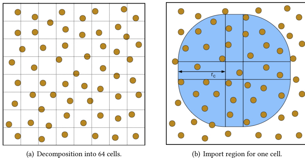
Figure 8.5: Spatial decomposition, showing particles in a 2-D computational box, (a) partitioned into 64 cells, (b) import region for one cell.
