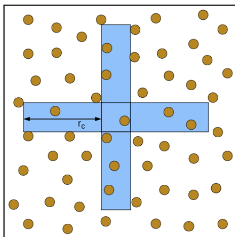
Figure 8.6: Neutral territory method, showing particles in a 2-D computational box and the import region (shaded) for one cell (center square). This Figure can be compared directly to the spatial decomposition case of Fig. 8.5(b). See Shaw [172] for additional details.
