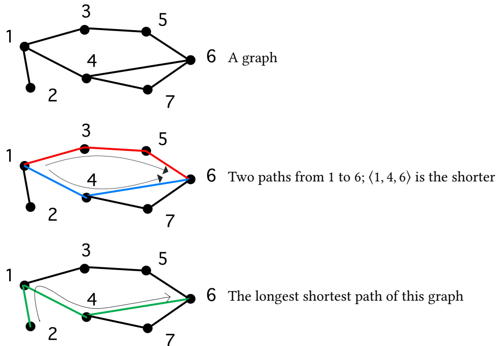
Figure 20.2: Shortest paths.
