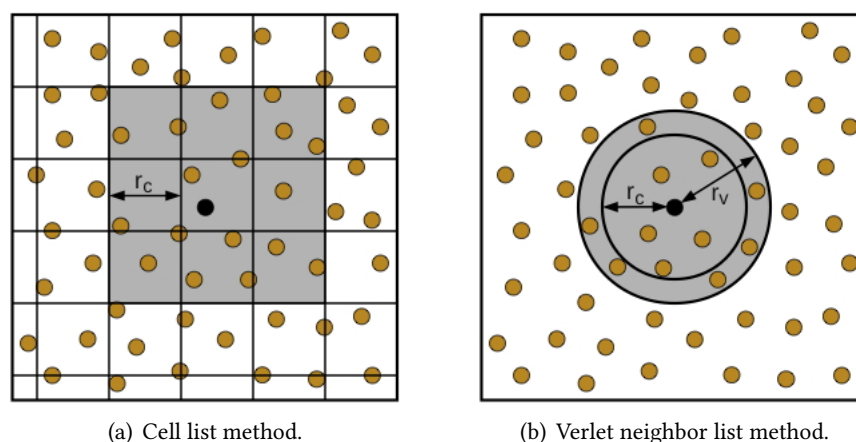
Figure 8.1: Computing nonbonded forces within a cutoff, r_c . To compute forces involving the highlighted particle, only particles in the shaded regions are considered.
