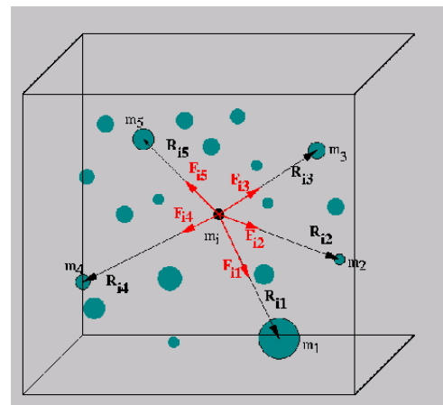
Figure 11.1: Summing all forces on a particle.
