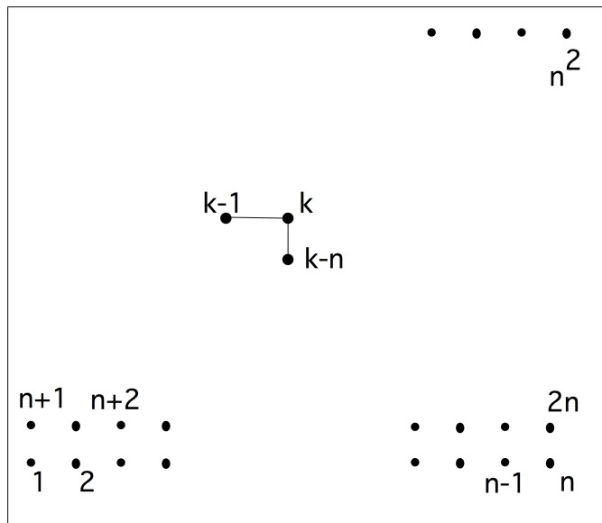
Figure 7.27: The difference stencil of the L factor of the matrix of a two-dimensional BVP.
