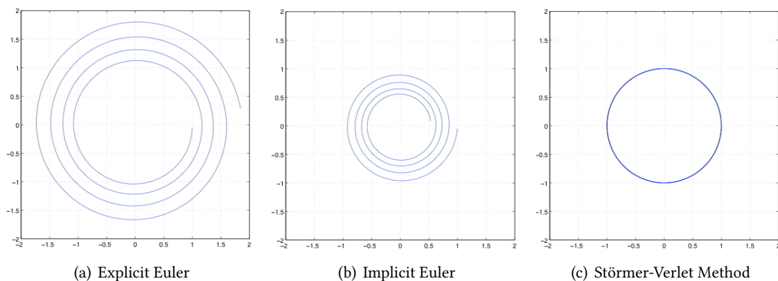
Figure 8.10: Phase plot of the solution of the simple harmonic oscillator for three methods with initial value (1, 0) , time step 0.05 , and 500 steps. For explicit Euler, the solution spirals outward; for implicit Euler, the solution spirals inward; the total energy is best preserved with the Störmer-Verlet method.
