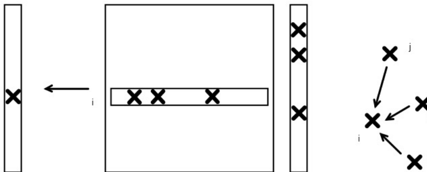
Figure 10.3: Pull model of graph algorithms, depicted in matrix-vector form
