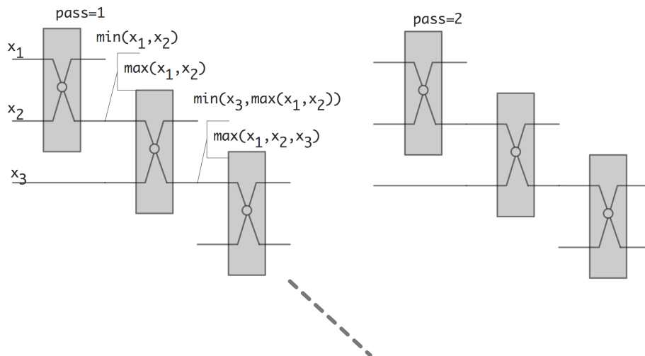
Figure 9.1: Bubble sort as a sorting network.
