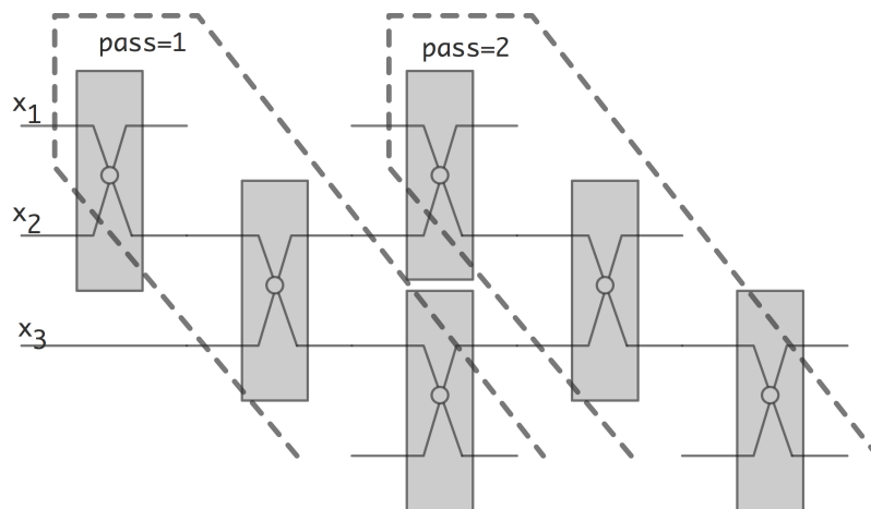
Figure 9.2: Overlapping passes in the bubble sort network.
