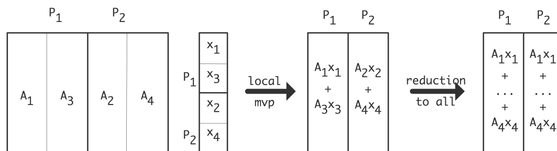
Figure 7.7: Matrix-vector multiplication with a cyclicly distributed matrix.
