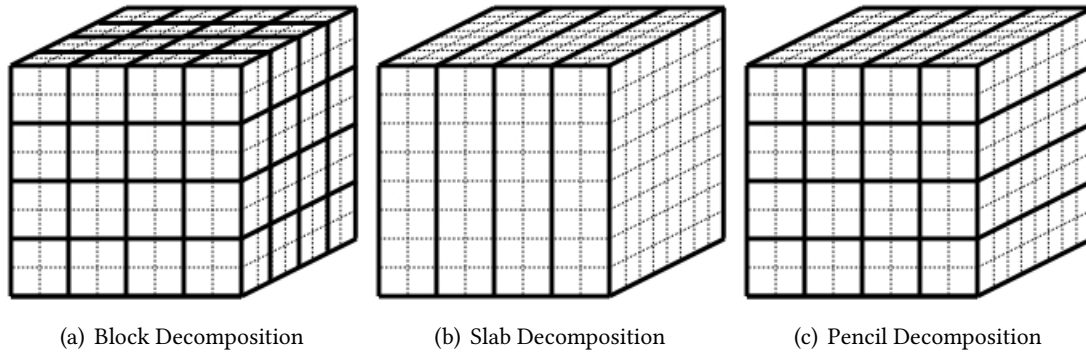
Figure 8.9: Three data decompositions for 3-D FFTs.
