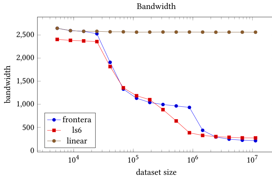
Figure 6.4: Single core bandwidth as function of data set size
