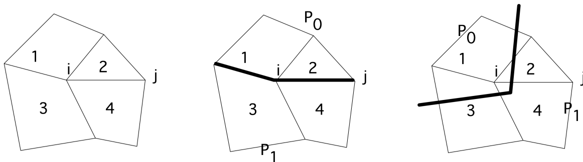
Figure 7.15: A finite element domain, parallelization of the matrix construction, and parallelization of matrix element storage.
