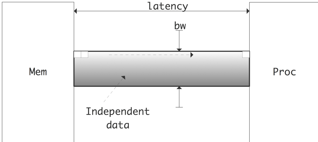
Figure 1.14: Illustration of Little's Law that states how much independent data needs to be in flight.
