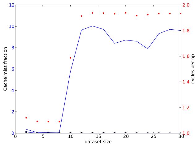
Figure 6.5: Average cycle count per operation as function of the dataset size.
