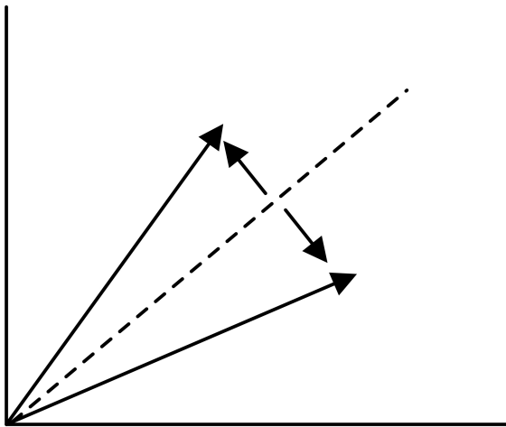
Figure 14.1: Householder reflector.
