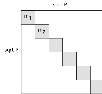
Figure 11.4: IMP realization of the 1.5D N-body problem.
