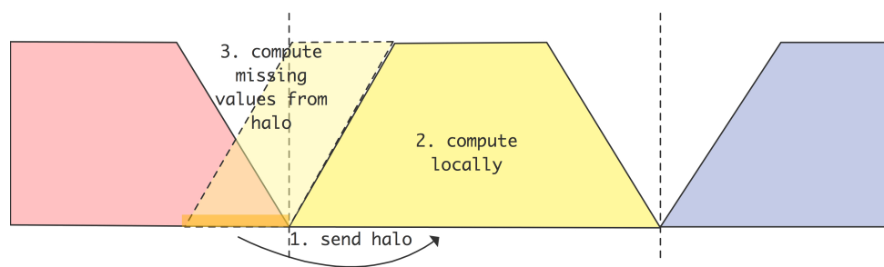
Figure 7.29: Computation of blocks of grid points over multiple iterations.
