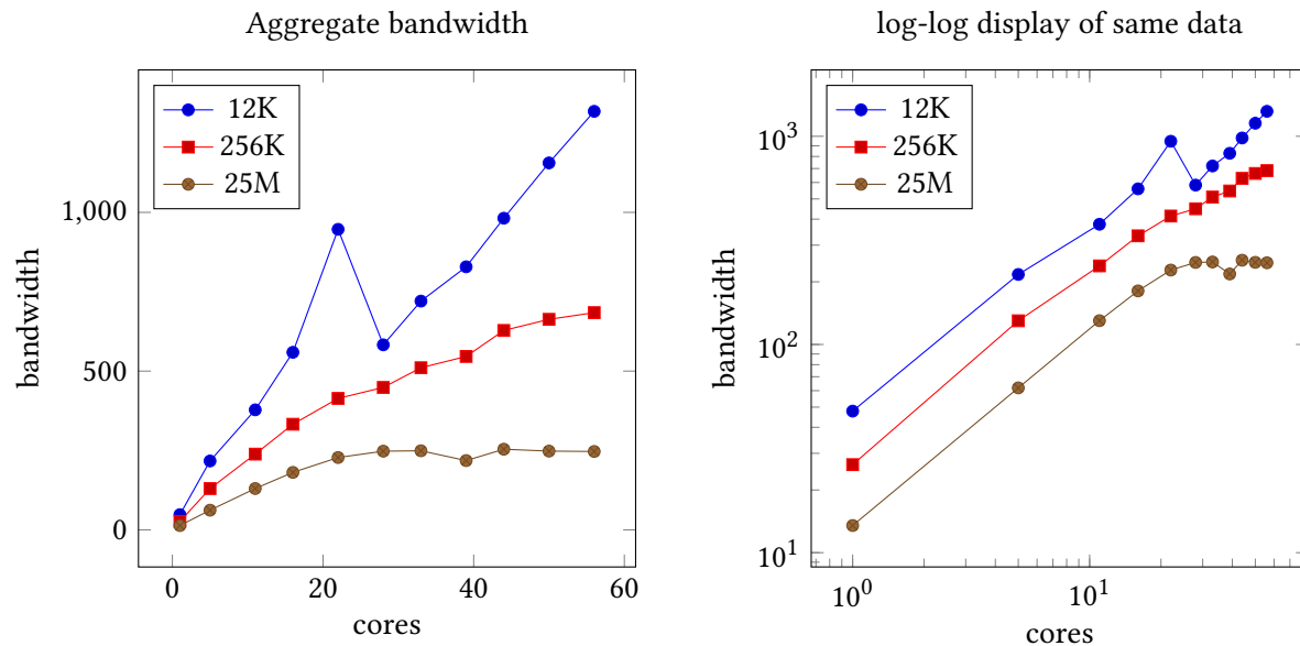
Figure 6.1: Aggregate bandwidth measurement as a function of core counts and data set sizes
