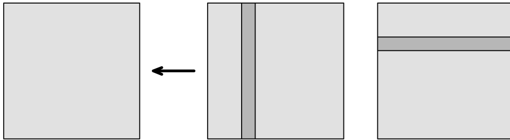
Figure 7.8: Matrix-matrix multiplication as a sequence of low-rank updates.
