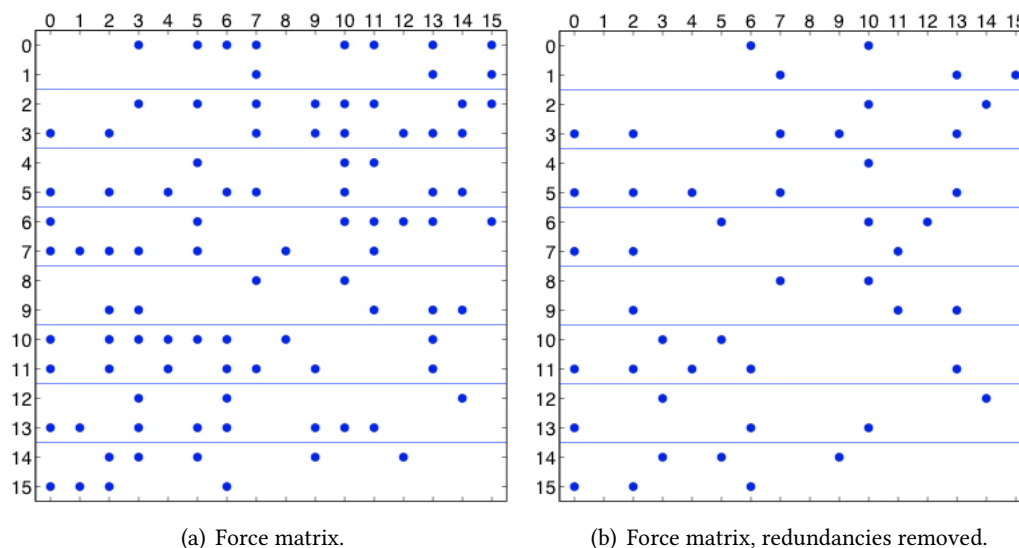
Figure 8.2: Atom decomposition, showing a force matrix of 16 particles distributed among 8 processors. A dot represents a nonzero entry in the force matrix. On the left, the matrix is symmetric; on the right, only one element of a pair of skew-symmetric elements is computed, to take advantage of Newton's third law.
