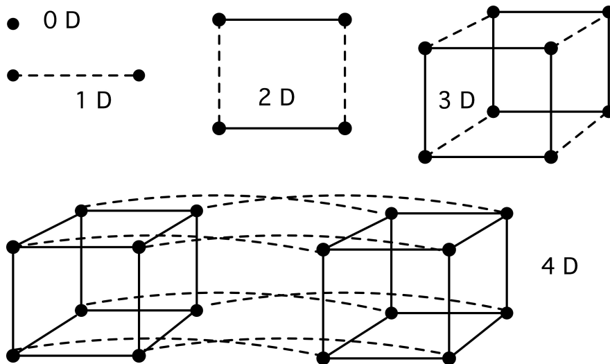
Figure 2.23: Hypercubes.
