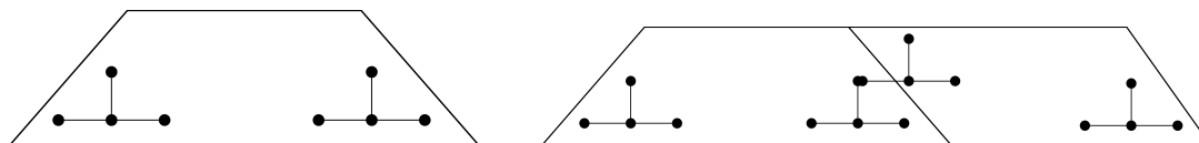
Figure 7.26: First and second step in cache-optimized iteration space traversal.
