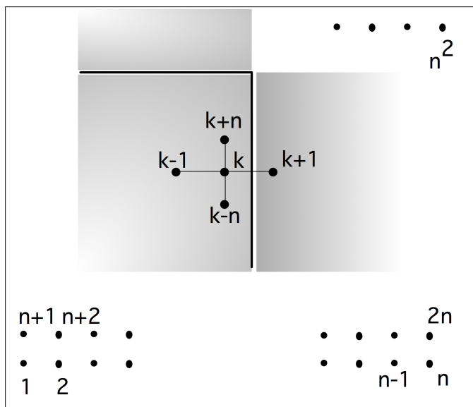
Figure 7.12: A difference stencil applied to a two-dimensional square domain, distributed over processors. A cross-processor connection is indicated..
