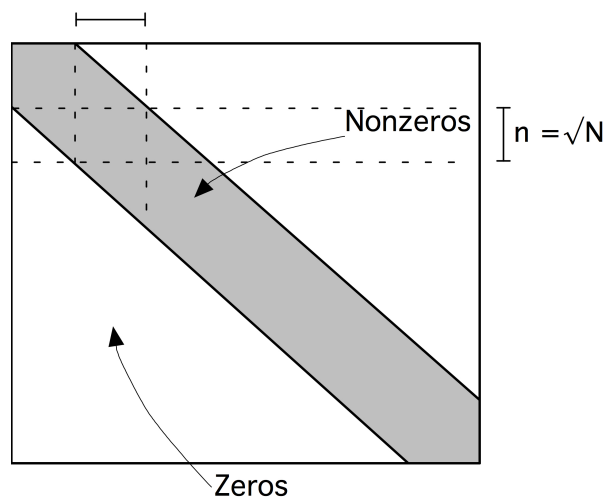
Figure 7.14: Band matrix with halfbandwidth \sqrt{N} .
