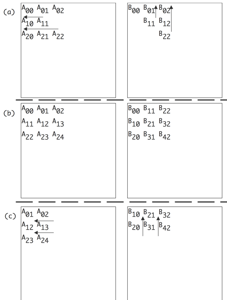
Figure 7.11: Cannon's algorithm for matrix-matrix multiplication: (a) initial rotation of matrix rows and columns, (b) resulting position in which processor (i, j) can start accumulating \sum_k A_{i,k} B_{k,j} , (c) subsequent rotation of A, B for the next term.
