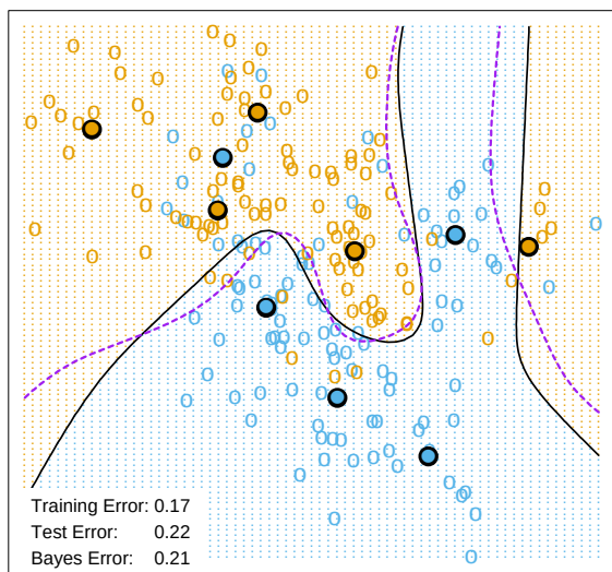
FIGURE 13.2. The upper panel shows the K -means classifier applied to the mixture data example. The decision boundary is piecewise linear. The lower panel shows a Gaussian mixture model with a common covariance for all component Gaussians. The EM algorithm for the mixture model was started at the K -means solution. The broken purple curve in the background is the Bayes decision boundary.
