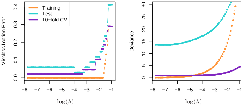
FIGURE 18.6. Training, test, and 10-fold cross validation curves for lasso logistic regression on the leukemia data. The left panel shows misclassification errors, the right panel shows deviance.
