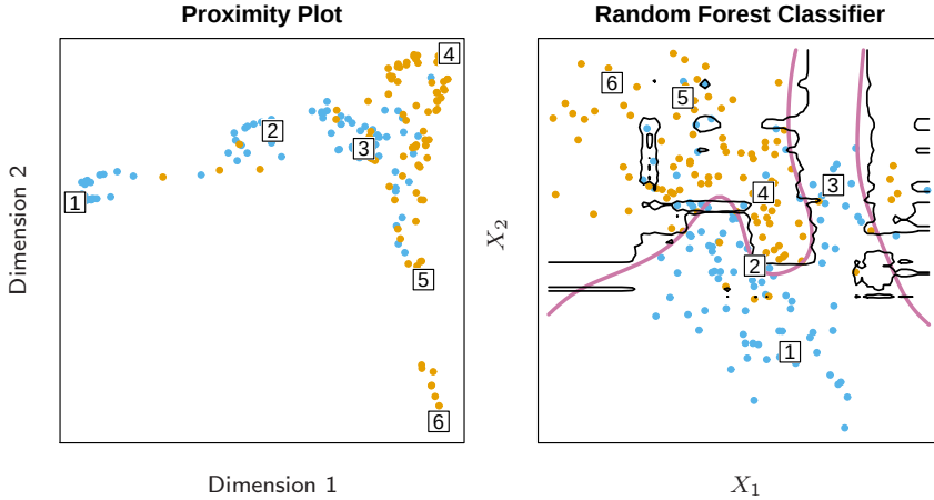
FIGURE 15.6. (Left): Proximity plot for a random forest classifier grown to the mixture data. (Right): Decision boundary and training data for random forest on mixture data. Six points have been identified in each plot.
