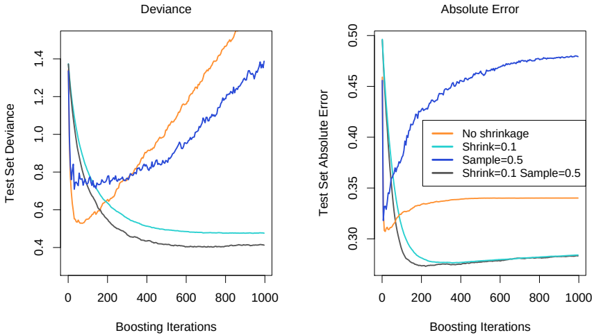
FIGURE 10.12. Test-error curves for the simulated example (10.2), showing the effect of stochasticity. For the curves labeled “Sample= 0.5”, a different 50% subsample of the training data was used each time a tree was grown. In the left panel the models were fit by gbm using a binomial deviance loss function; in the right-hand panel using square-error loss.
