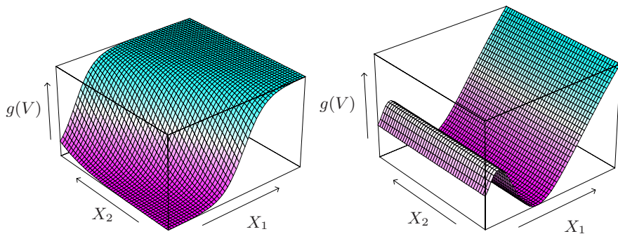
FIGURE 11.1. Perspective plots of two ridge functions.
