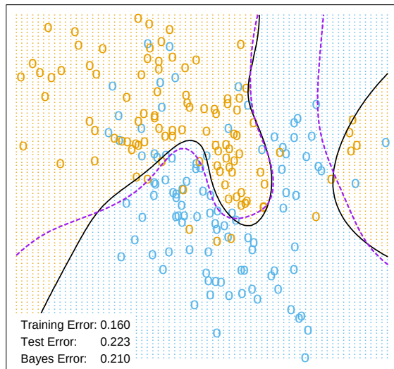
FIGURE 11.4. A neural network on the mixture example of Chapter 2. The upper panel uses no weight decay, and overfits the training data. The lower panel uses weight decay, and achieves close to the Bayes error rate (broken purple boundary). Both use the softmax activation function and cross-entropy error.
