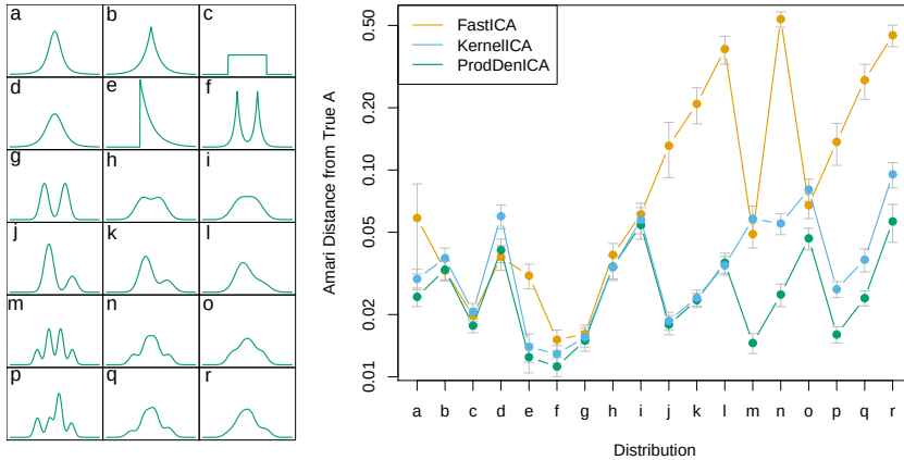
FIGURE 14.42. The left panel shows 18 distributions used for comparisons. These include the “t”, uniform, exponential, mixtures of exponentials, symmetric and asymmetric Gaussian mixtures. The right panel shows (on the log scale) the average Amari metric for each method and each distribution, based on 30 simulations in \mathbb{R}^2 for each distribution.
