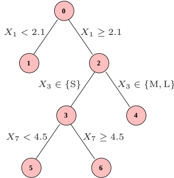
FIGURE 16.9. A typical tree in an ensemble, from which rules can be derived.
