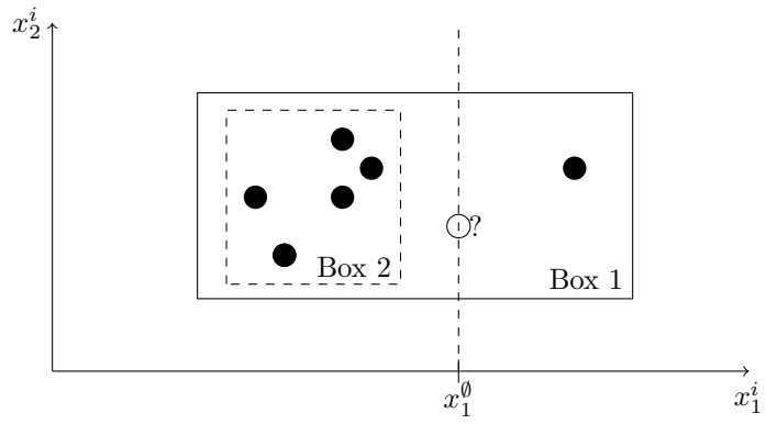
Figure 1: Example of database with one very negative point \mathbf{x}^0 given by the non-filled circle with its missing coordinate. Other points are positives. If \mathbf{x}^0 is removed from the database, the candidate box is box 1. The optimal box is box 2 which is obtained if we consider \mathbf{x}^0 included in dimension 2.
